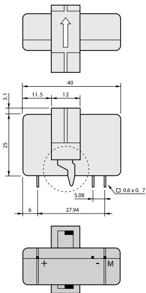
EL...BB current sensors
