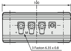
Size 1 - CS500BR and CS1000BR
